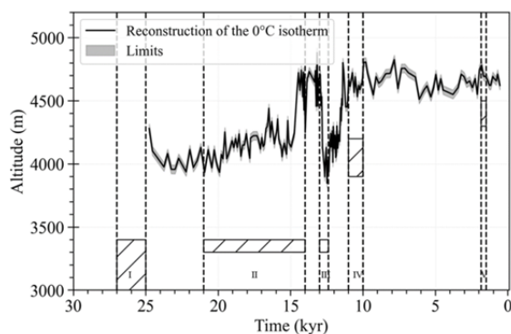
Fig. 7 Likely average lowering of the FLH in the southwestern flank of the Sierra Nevada del Cocuy. The solid line depicts the inferred mean value. The gray shading represents the upper and lower limits. Phases of glacier expansion in the Sierra Nevada (van der Hammen et al. 1980/1981) are highlighted with vertical dashed lines: (I) Cóncono, 27 to 25 kyr; (II) Early Lagunillas, 21 to 14 kyr; (III) Late Lagunillas, 13 to 12.4 kyr; (IV) Bocatoma, 11 to 10 kyr; and (V) Corralitos, 1500 to 1850 C.E. The striped boxes depict the ranges of heights suggested by van der Hammen et al. (1980/1981) for past glacier-front advances.
