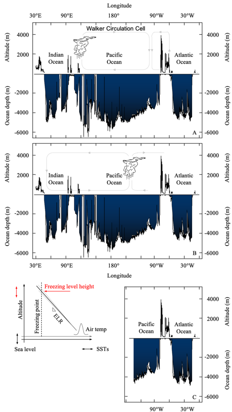
Fig. 2 Topographic profile along a 5°N zonal transect extending from 30°E to the Greenwich Meridian. (A) December-January-February (DJF) East-West circulation in the equatorial troposphere during normal conditions. (B) DJF East-West circulation during El Niño-like conditions. The black solid line depicts the ground surface (above the mean sea level) and the ocean bottom (below the mean sea level) along the 5°N transect. The gray solid lines and the blue shaded areas represent the circulation cells and the oceans, respectively. (C) Schematic diagram of the method implemented and data required (left sketch) to assess long-term fluctuations in the freezing level height. Inferred altitudes of the 0°C isotherm are projected on the upper ranges of the Andes Cordillera – see sketch to the right.
