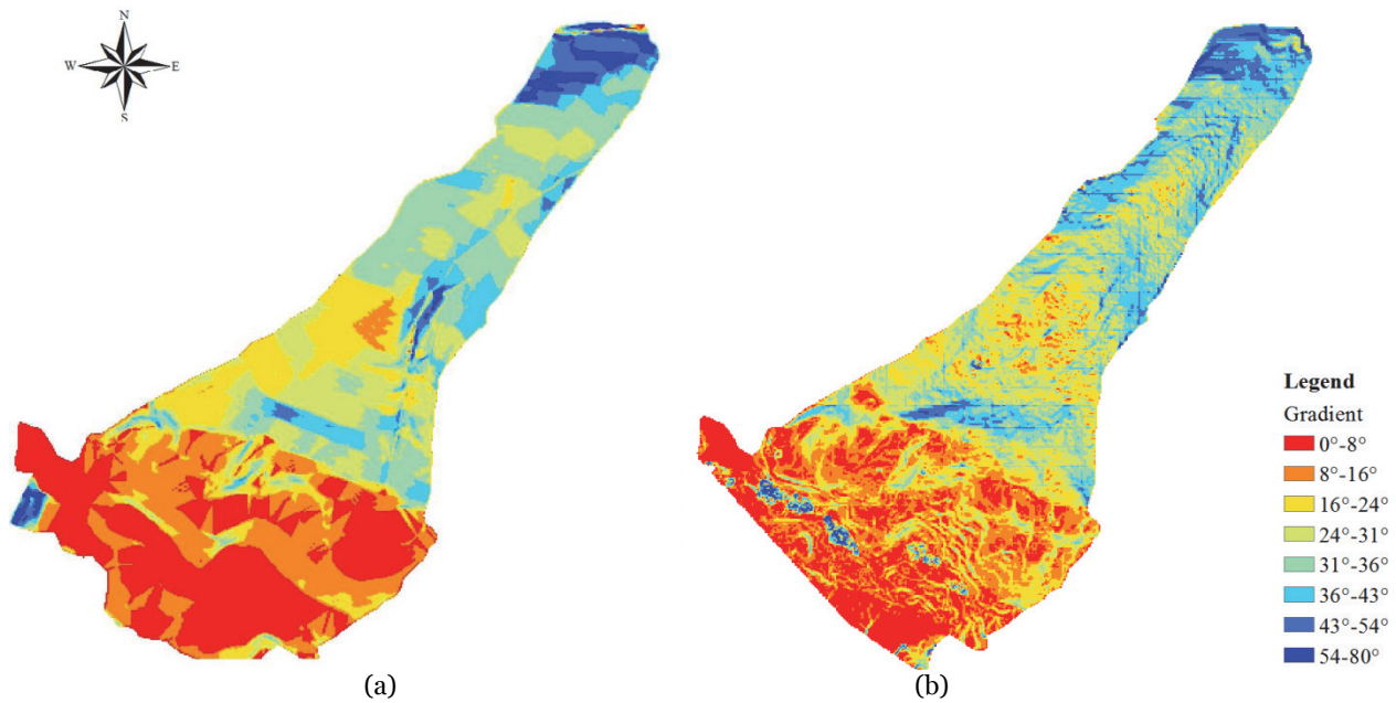
Figure 7 Distribution of local slope gradients before (a) and after (b) the landslide.
