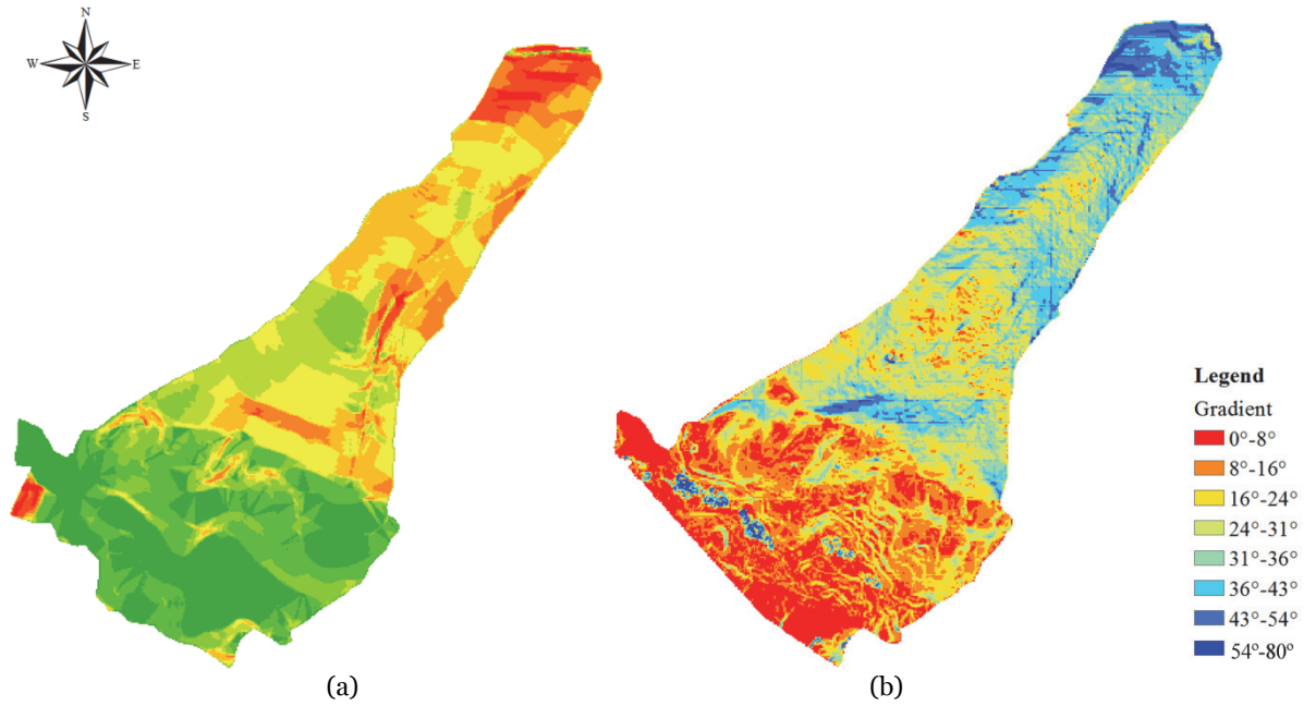
Figure 7 Distribution of local slope gradients before (a) and after (b) the landslide.
